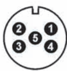
5 pins M12 connector (View toward sensor pins)
